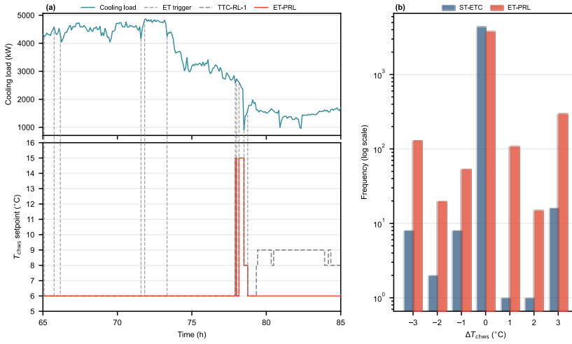
Figure 6 Local event triggered response and global difference frequency statistics. Panel a shows the cooling load and absolute setpoint trajectories from 65 h to 85 h, and panel b shows the logarithmic frequency distributions of \Delta T_{chws} for ST-ETC and ET-PRL relative to TTC-RL-1
