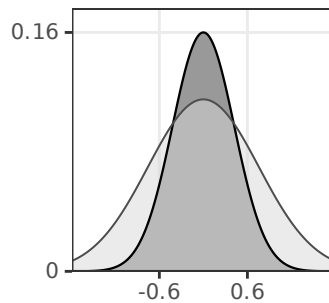
Convolved Cross-Section
