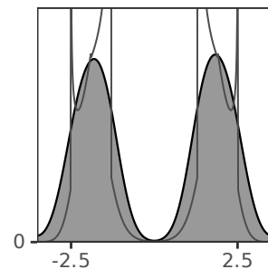
Symplectic Resolution
