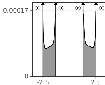
Semiclassical Caustics
