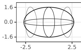
Phase-Space Cells
