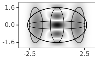
Phase-Space Cells
