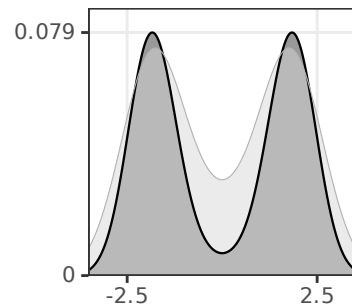
Symplectic Resolution
