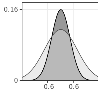
Convolved Cross-Section
