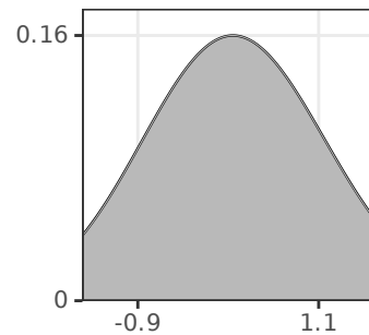
Symplectic Resolution
