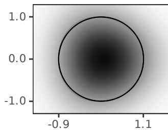
Phase-Space Cells
