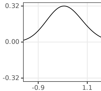
Wigner Negativity
