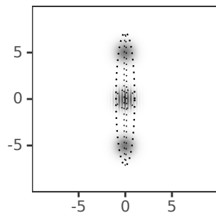
Phase-Space Cells
