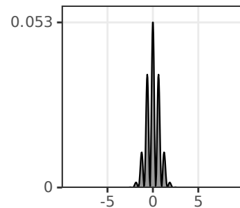
Symplectic Resolution
