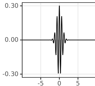
Wigner Negativity
