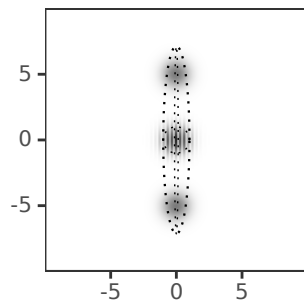
Phase-Space Cells
