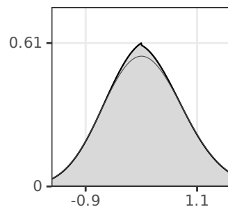
Airy Approximation
