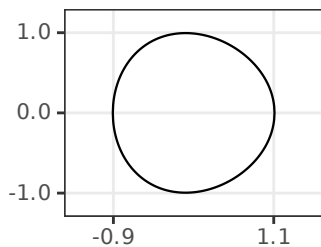
Classical Orbit
