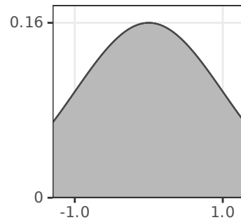
Symplectic Resolution
