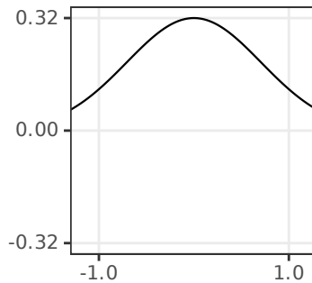
Wigner Negativity
