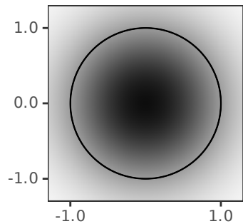
Phase-Space Cells
