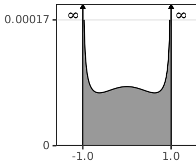
Semiclassical Caustics
