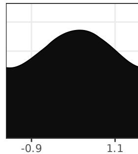
Symplectic Resolution
