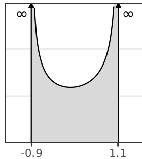
Semiclassical Caustic:
