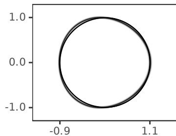
Phase-Space Cells
