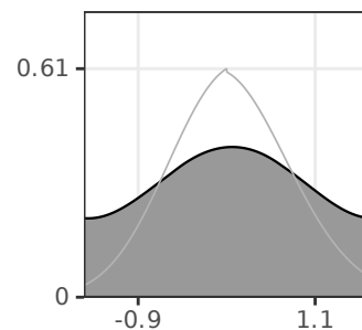
Symplectic Resolution
