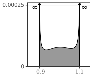
Semiclassical Caustics
