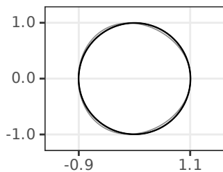
Phase-Space Cells
