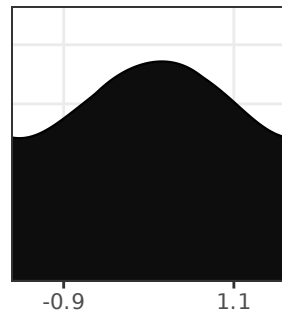
Symplectic Resolution
