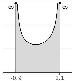
Semiclassical Caustics
