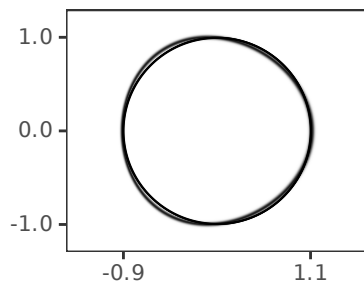
Phase-Space Cells
