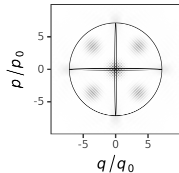
Zurek compass ( \max|D|=0.21 )
