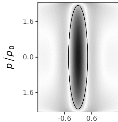
Squeezed vacuum ( \max|D|=0.13 ) Harmonic n=1 ( \max|D|=0.2 )
