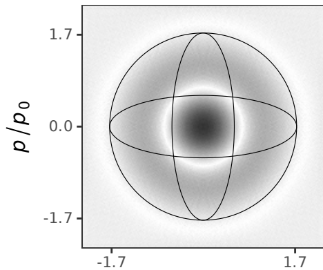
Squeezed vacuum ( \max|D|=0.13 ) Harmonic n=1 ( \max|D|=0.2 )
