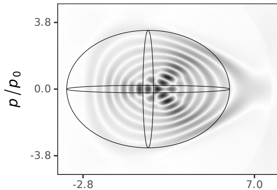
Morse n=8 ( \max|D|=0.12 )
