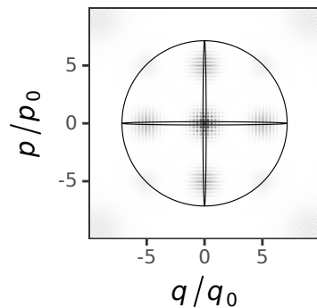
4-cat square ( \max|D|=0.21 )
