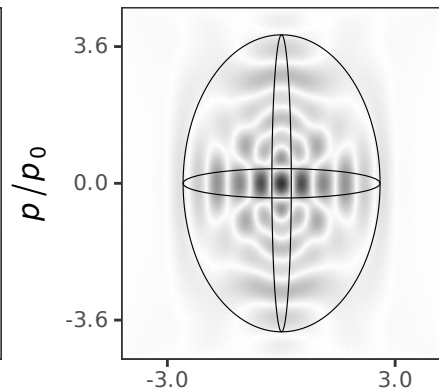
Double-well n=5 ( \max|D|=0.18 )
