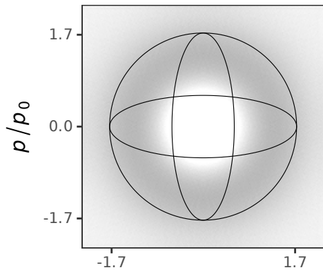
Squeezed vacuum (min=-0.0099)
