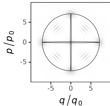
Zurek compass (min=-0.089)
