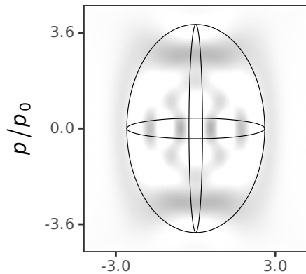
Double-well n=5 (min=-0.14)
