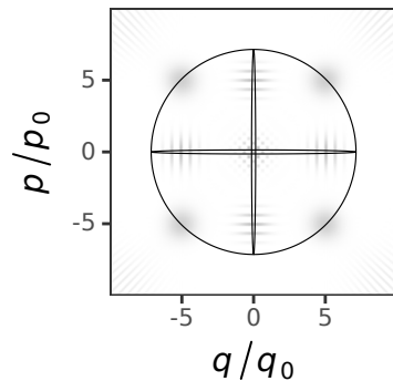
4-cat square (min=-0.09)
