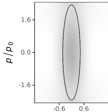
Squeezed vacuum (min=-0.0099)
