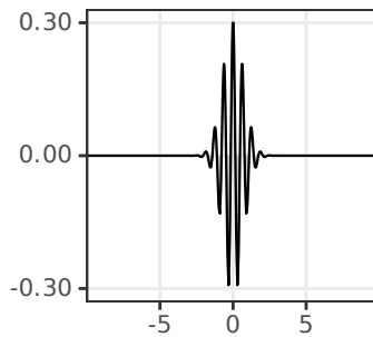
Wigner Cross-Section
