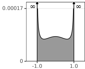
Semiclassical Caustics
