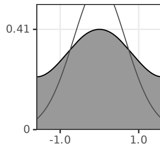
Symplectic Resolution
