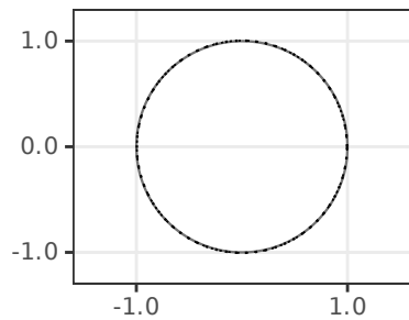
Phase-Space Cells
