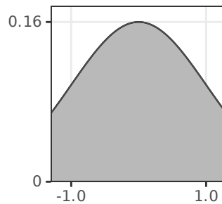
Symplectic Resolution
