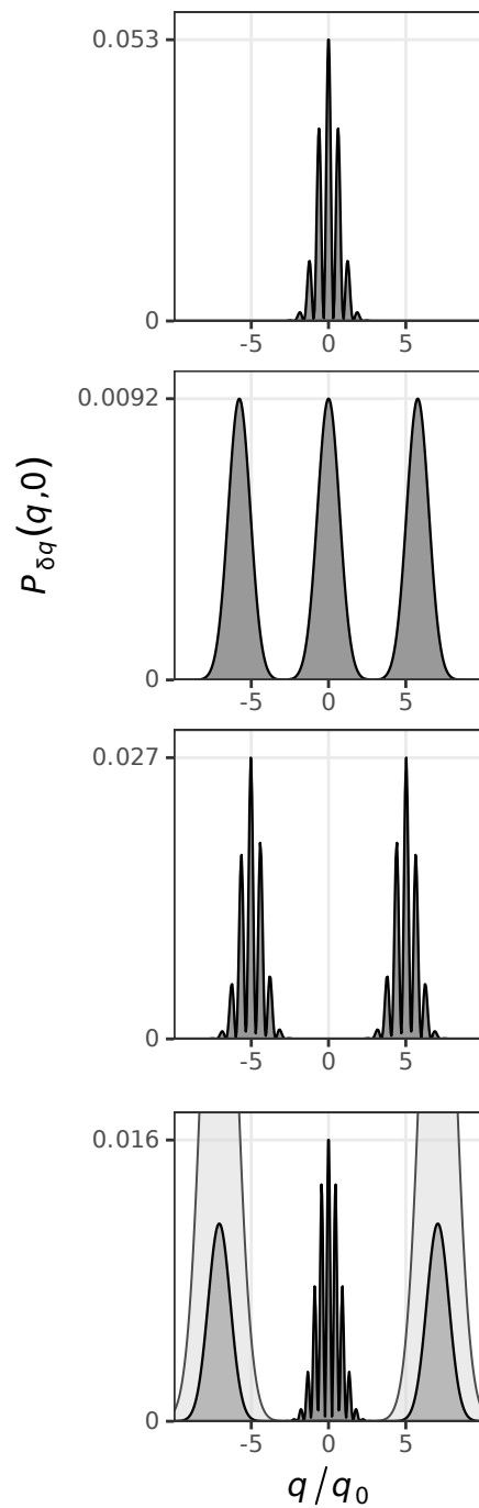
Symplectic Resolution
