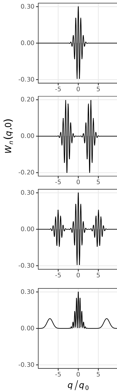
Wigner Negativity
