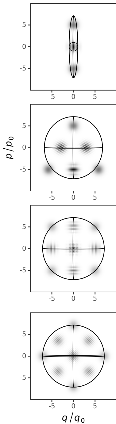
Phase-Space Cells
