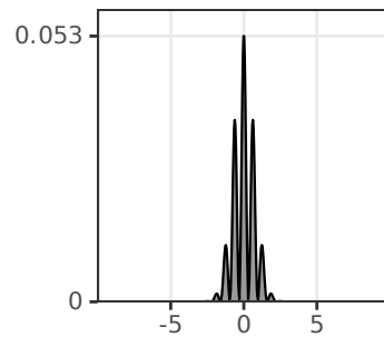
Convolved Cross-Section
