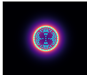
QHO n=20
