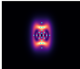
Double-well
