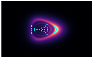
Morse
