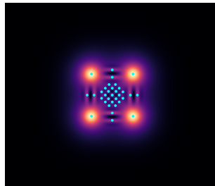
4-cat diag
