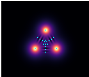
3-cat
