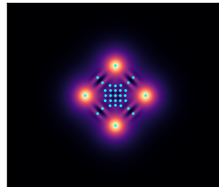
Compass
