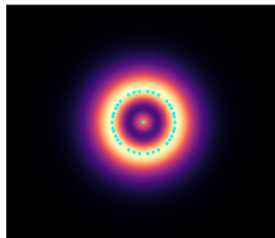
QHO n=2
