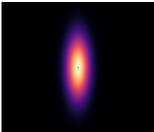
Squeezed
