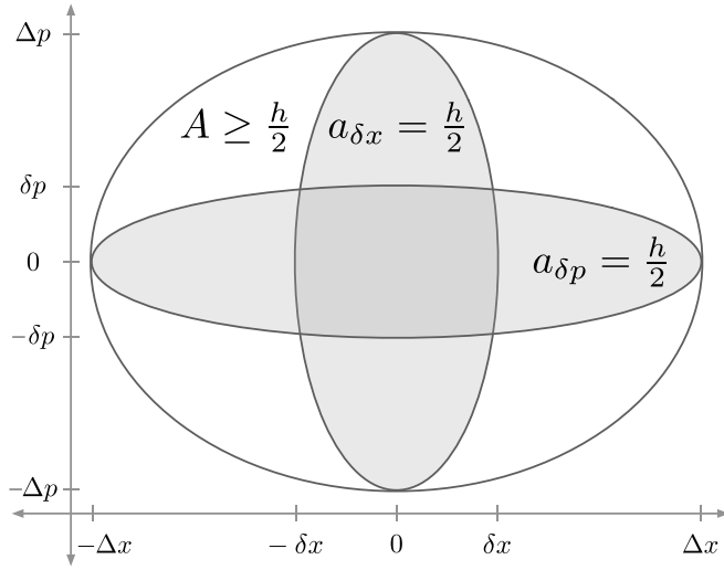
FIG. 2. Zurek cells
