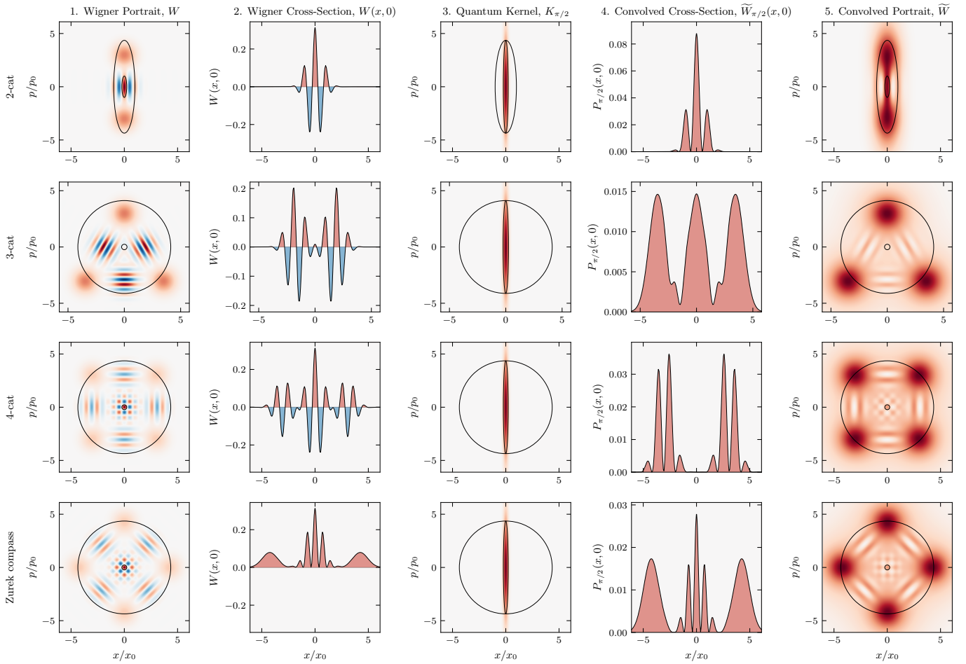
FIG. 5. Cat states. Rows correspond to the 2-cat, 3-cat, 4-cat, and Zurek compass states. Columns are as in Fig. 3. As before, the portrait \tilde{W} (Column 5) is everywhere non-negative, with positive lobes matching the count and location of those in W , resolved at scale \tilde{a} . The 4-cat and Zurek compass states differ by a \pi/4 rotation in phase space.
