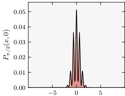
Convolved Cross-Section
