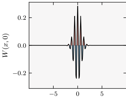
Wigner Cross-Section
