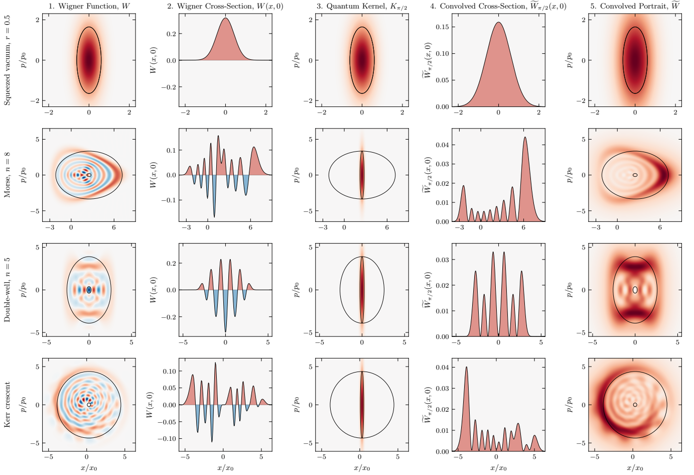
FIG. 5. Squeezed vacuum, eigenstates, and the Kerr crescent. Rows correspond to the squeezed vacuum ( r = 0.5 ), the Morse eigenstate ( n = 8 ), the double-well eigenstate ( n = 5 ), and the Kerr crescent, a coherent state sheared at constant photon number. Columns are as in Fig. 3. The Kerr state is shown in the principal frame of its covariance, where the overlays are axis-aligned. The portrait \tilde{W} (Column 5) remains strictly non-negative across all four states, resolved at a .
