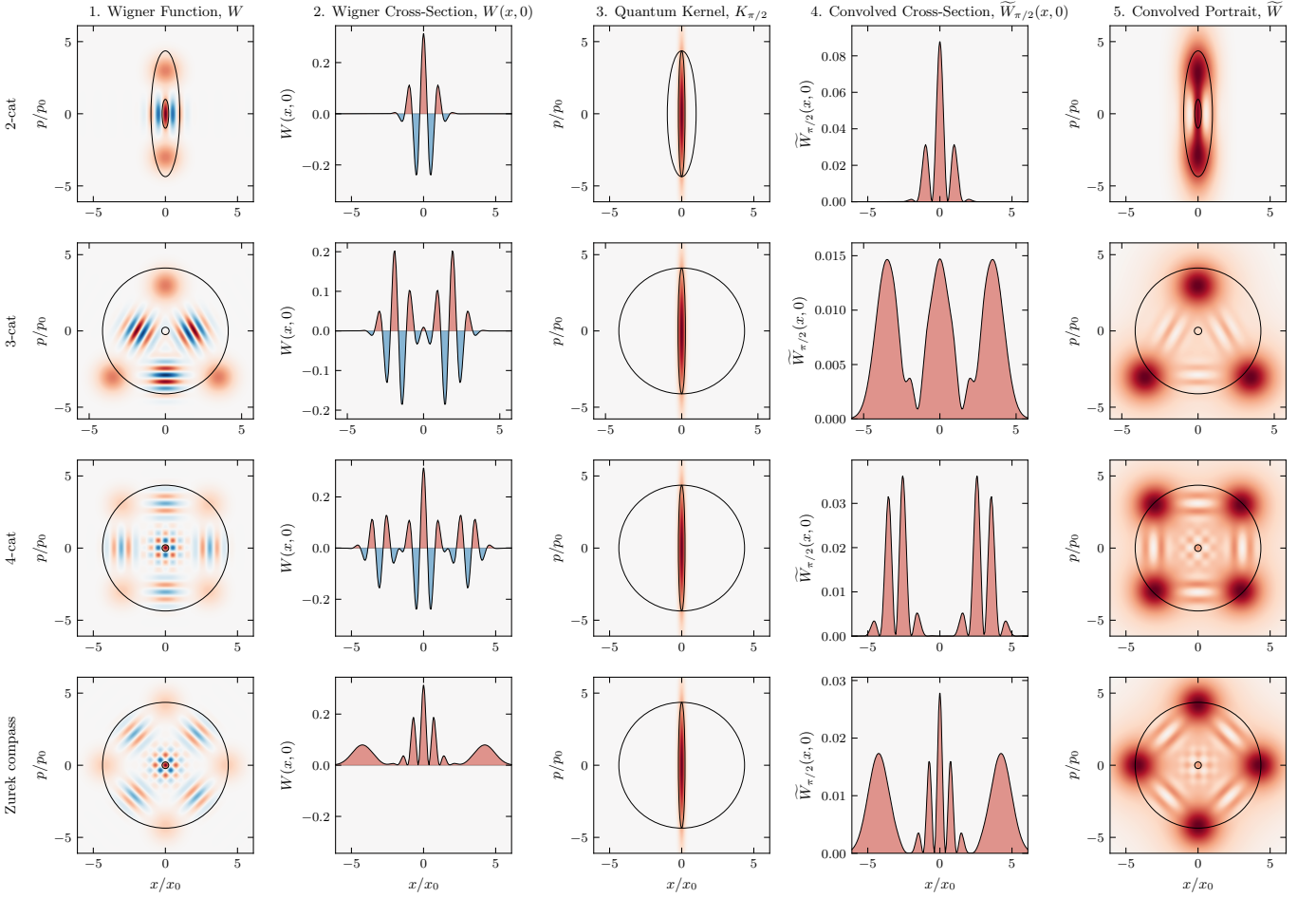
FIG. 4. Cat states. Rows correspond to the 2-cat, 3-cat, 4-cat, and Zurek compass states. Columns are as in Fig. 3. As before, the portrait \tilde{W} (Column 5) is everywhere non-negative, with positive lobes at the positions of those in W , resolved at a . The 4-cat and Zurek compass states differ by a \pi/4 rotation in phase space.
