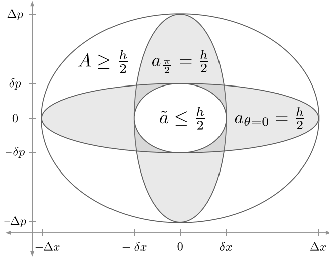
FIG. 1. Heisenberg cell, principal quantum blobs, and quorum cell. The Heisenberg cell is the state's covariance ellipsoid with action capacity A = \pi \Delta x \Delta p \geq h/2 . The quantum blob family (Fig. 2) has two members at the principal axes, a_{\theta=0} = \pi \Delta x \delta p = h/2 and a_{\pi/2} = \pi \delta x \Delta p = h/2 . Zurek's relations \delta p \sim \hbar/\Delta x and \delta x \sim \hbar/\Delta p locate the semi-axis scales from the state's action capacity. The quorum cell \tilde{a} is an ellipse with semi-axes \delta x, \delta p and action \tilde{a} = \pi \delta x \delta p . A circumscribes a_{\theta=0} and a_{\pi/2} , which circumscribe \tilde{a} .
