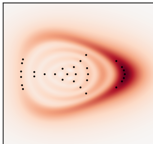
3-cat
