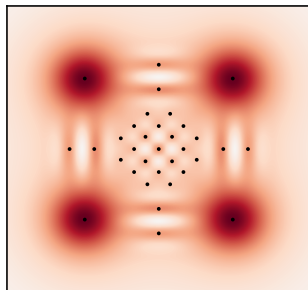
4-cat diag
