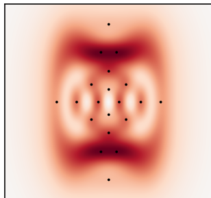
4-cat diag
