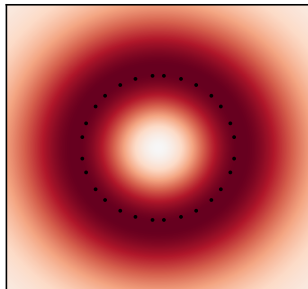
Morse
