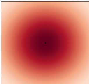
Squeezed
