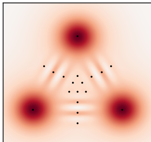
3-cat
