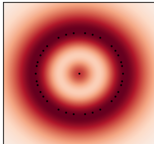
Double-well
