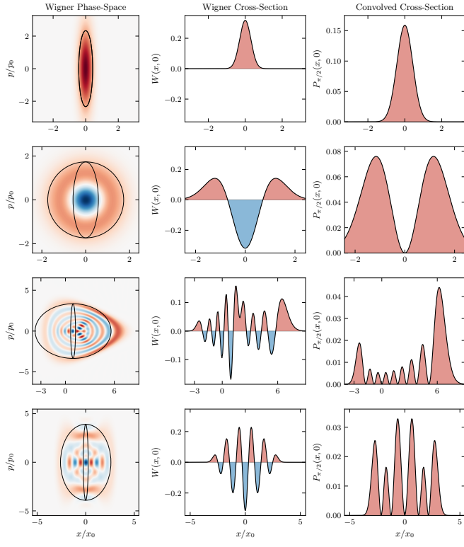
FIG. 1. Squeezed vacuum ( r = 0.5 ), harmonic oscillator n = 1 , Morse n = 8 , and double-well n = 5 .
