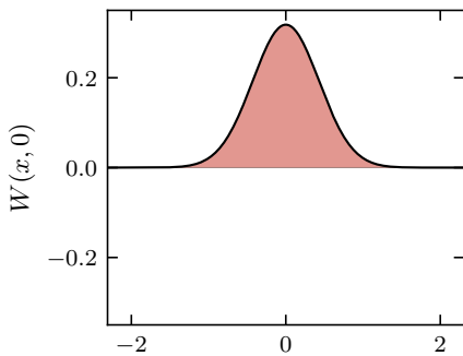
Wigner Cross-Section
