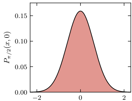
Convolved Cross-Section
