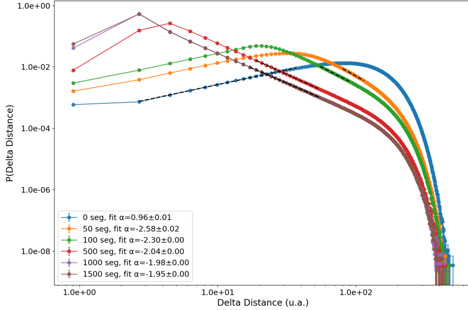
Figure 13: Displacement distribution for the second model, with constant rest time.
