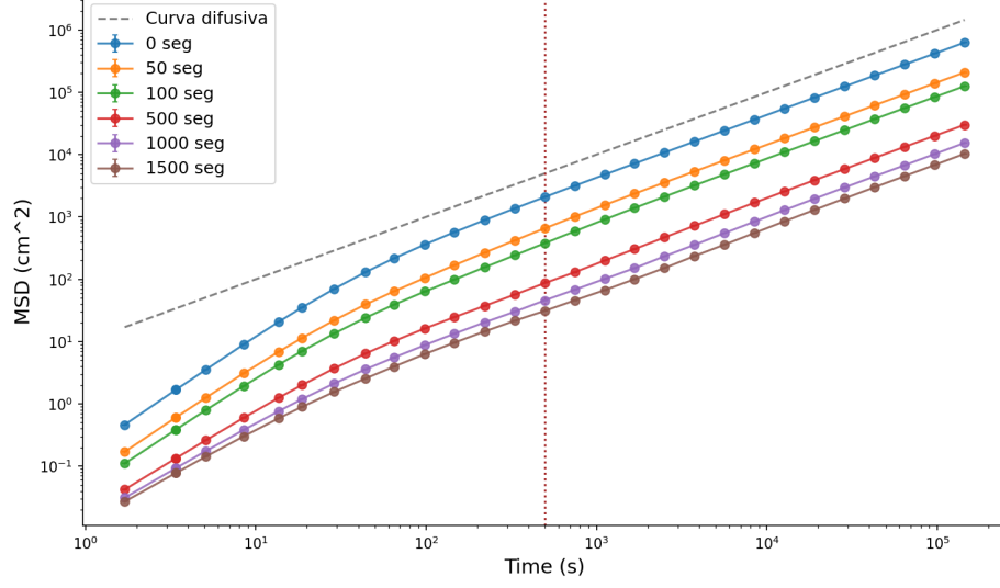
Figure 14: MSD for the second model, with constant rest time.
