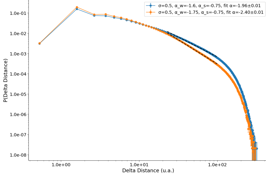
Figure 16: 15-minute displacement distribution for \sigma_\theta = 0.5 , \alpha_S = 0.75 and \alpha_W = 1.6 and 1.75 .
