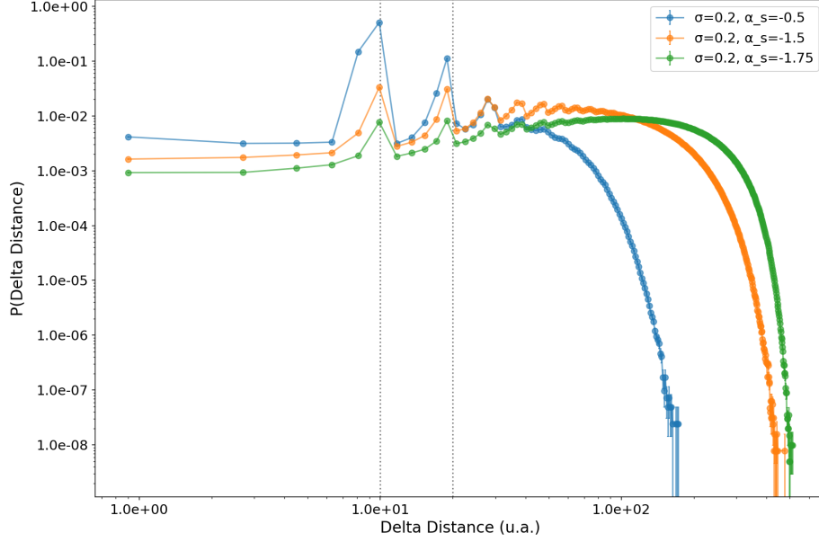
Figure 12: Displacement distribution for the first model, with constant walking time.
