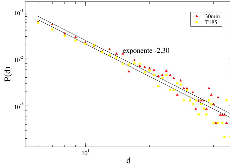
Figure 19: Distribution of traveled distances for T185, using \Delta t = 15 min and \Delta t = 30 min.
