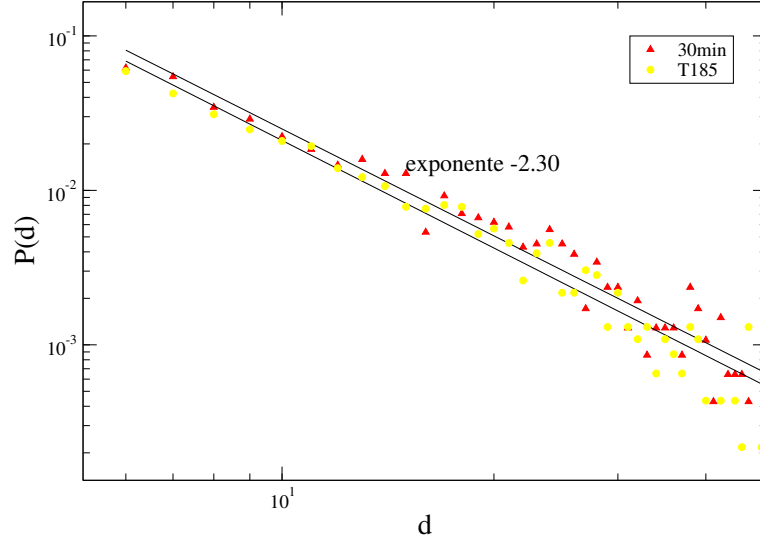
Figure 18: Distribution of traveled distances for T185, using \Delta t = 15 min and \Delta t = 30 min.
