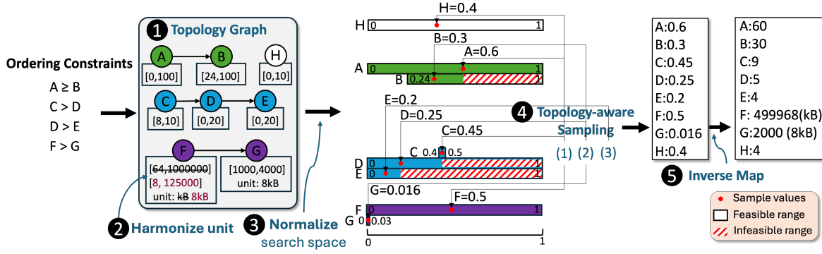
Figure 3: End-to-end illustration of the exploration phase. Given four ordering constraints, including a chained dependency ( C > D > E ), we construct the topology graph, where independent knob H appears as an isolated node. Heterogeneous units (e.g., F and G ) are harmonized to enable consistent comparison, and each connected component (color-coded) is normalized via component-wise min-max normalization while preserving relative structure. Topology-aware sampling generates a feasible configuration in three steps by respecting dependency order and feasible ranges. Finally, normalized values are mapped back to knob units through inverse transformation.
