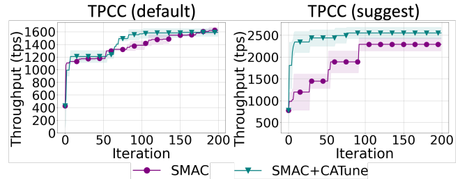
Figure 6: Best performance achieved by CATUNE under manual default ranges and knowledge-guided ranges on TPC-C on MySQL.
