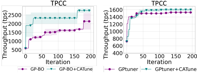
Figure 7: Performance of CATUNE integrated with GP-BO under knowledge-guided suggested ranges.
