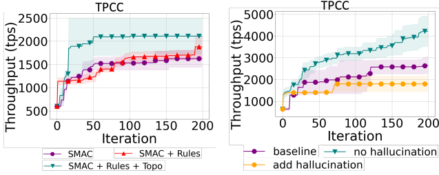
Figure 10: The result of ablation study for CATUNE, studying different constraint handling strategies.
