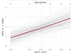
M_best (long_no. freq. slopes): per-child trajectory fan
