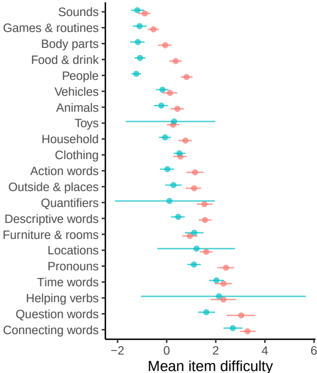
Semantic category
