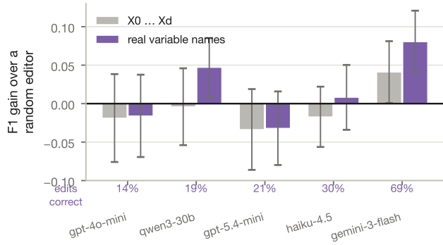
(b) real names, scarce data: it finally does
