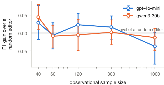
(a) anonymized variables: an edge only at n = 40
