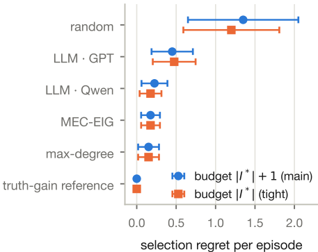
(a) selection regret (lower better)
