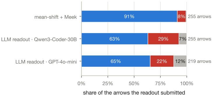
(a) submitted arrows by outcome
