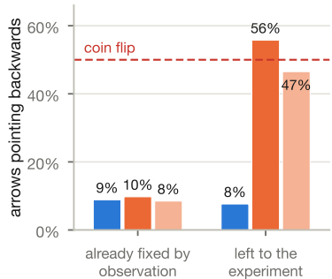
(b) reversal rate by decision source
