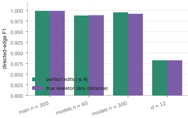
(a) synthetic: the edit budget never binds
