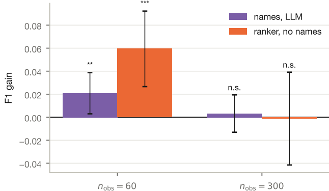
(b) names help, statistics help more
