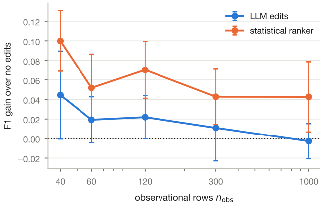
(a) only where the estimator is underpowered
