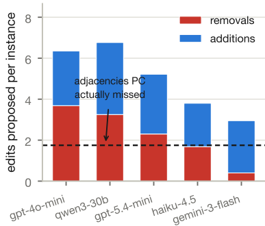
(a) how much they propose
