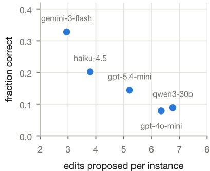
(c) restraint, not volume
