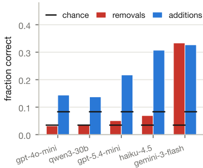
(b) and how often they are right
