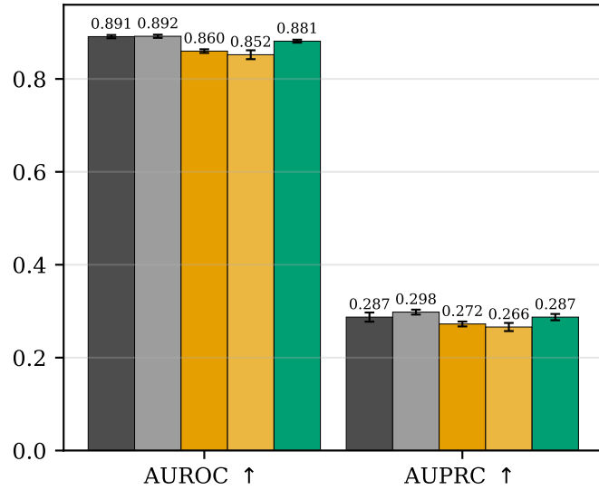
PTB-XL
