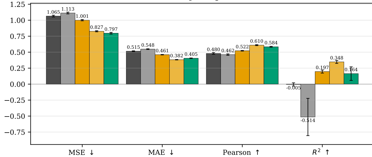
Aionoscope (regression)
