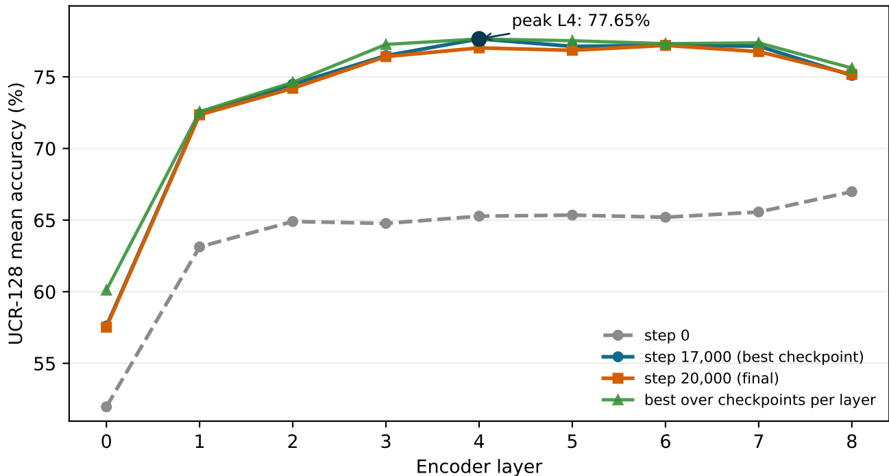
LeNEPA UCR layer profile: middle layers dominate
