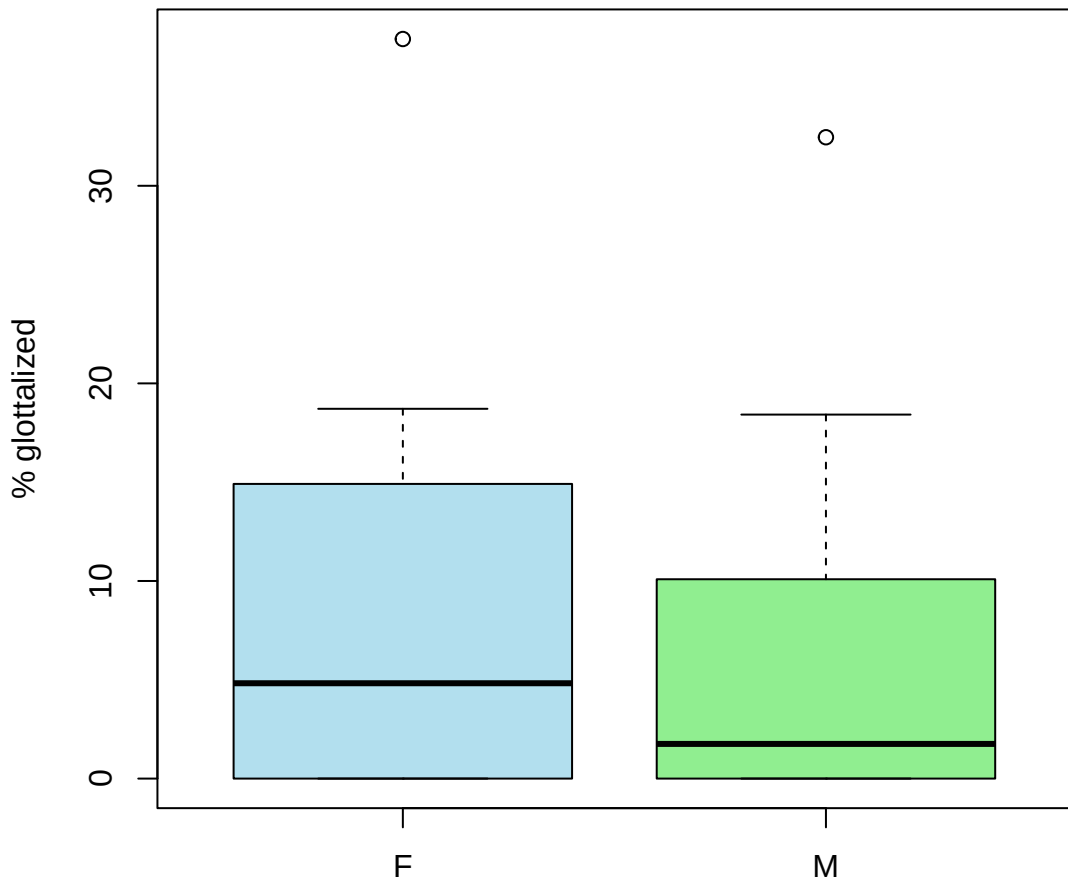
% glottalized, by sex
