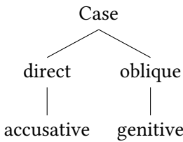
Figure 2.1: Hierarchy of case features
