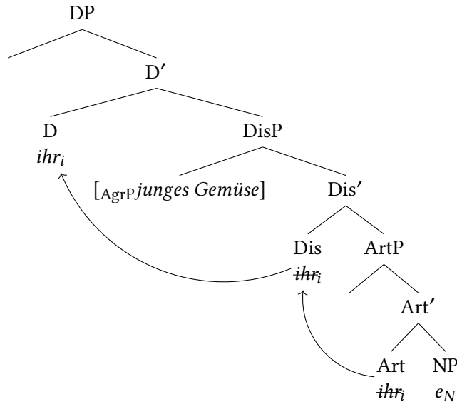
Figure 2.27: Intransitive pronouns (Dis-agreement)
