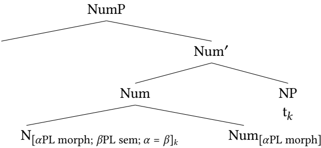
Figure 7.6: General makeup of nouns
