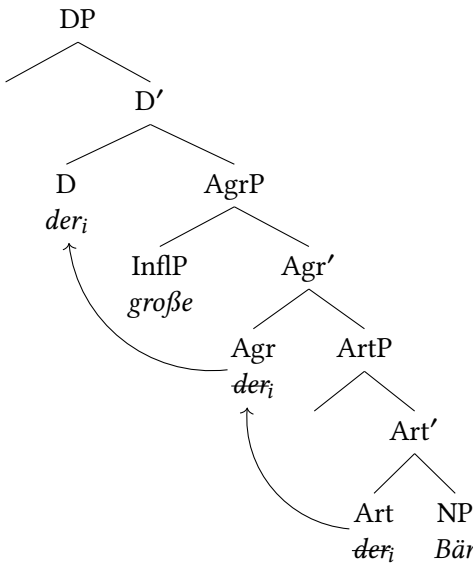
Figure 2.21: Regular DP-structure (Simplified)
