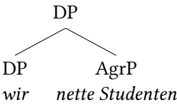
Figure 3.6: Pronominal DP – high right-adjunction
