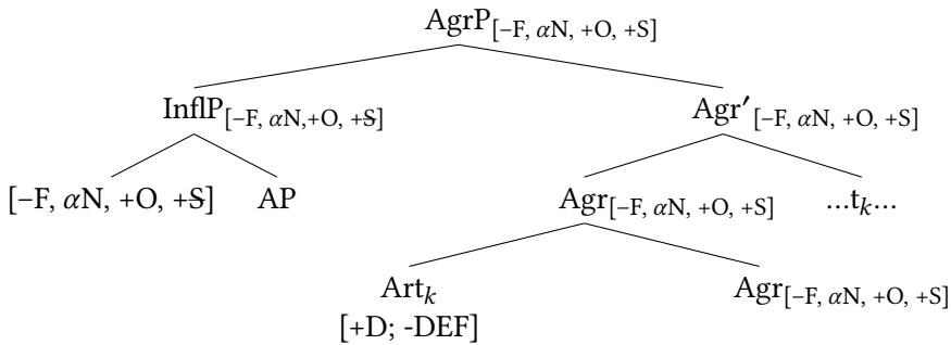
Figure 2.15: Percolation of reduced features
