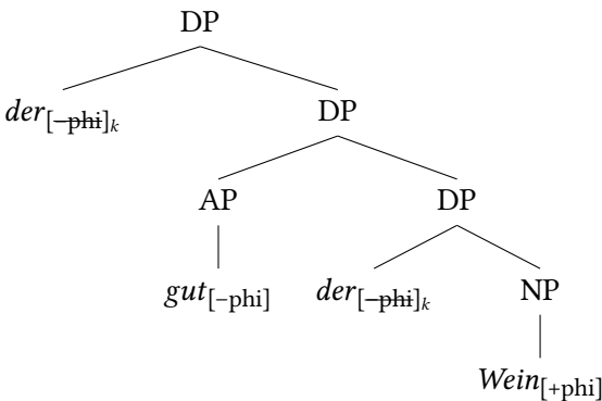
Figure 2.36: der gut-e Wein the good-ST wine.MASC 'the good wine'
