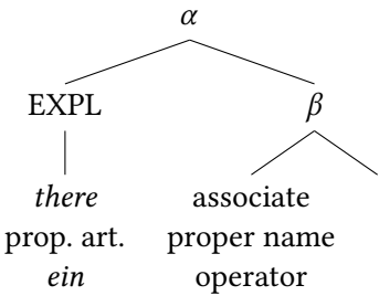
Figure 8.6: Structural relation between expletives and substantive elements
