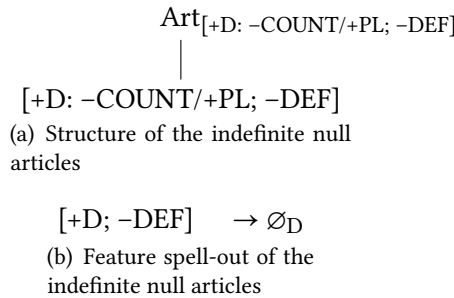
Figure 8.2: Indefinite null articles
