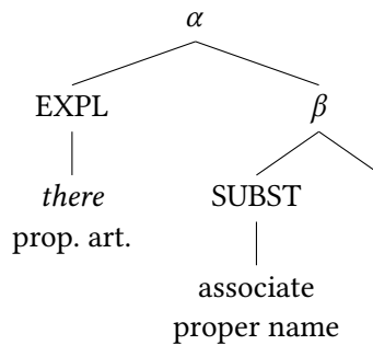
Figure 1.1: Structural relation between expletives and substantive elements
