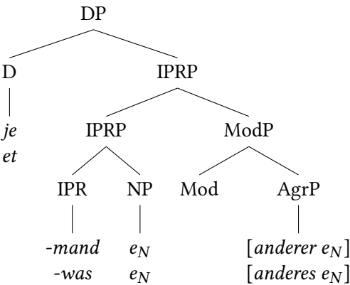
Figure 3.1: Indefinite pronoun construction
