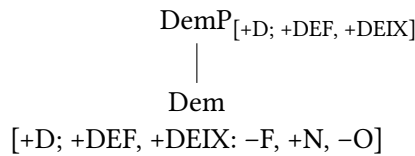
Figure 4.9: Structure of uninflected dies
