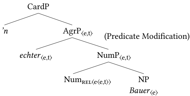
Figure 6.7: Intensified comparative reading in TP Du bist vielleicht 'n echter Bauer! you are PRT a real peasant.MASC 'You are really like a peasant!'
