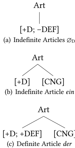
Figure 1.4: Structures of articles
