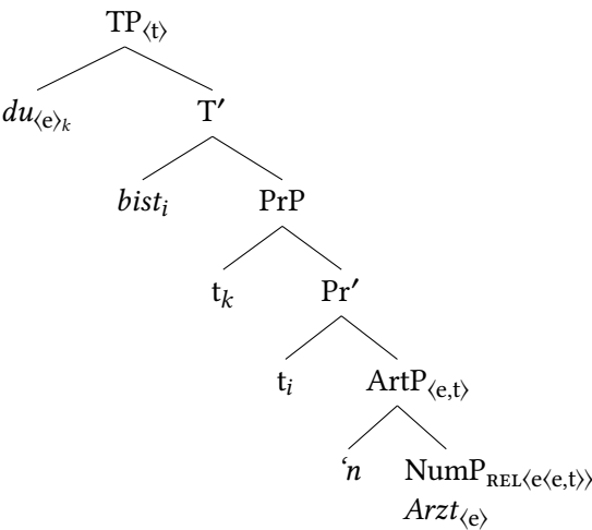
Figure 7.5: Agreement in the TP
