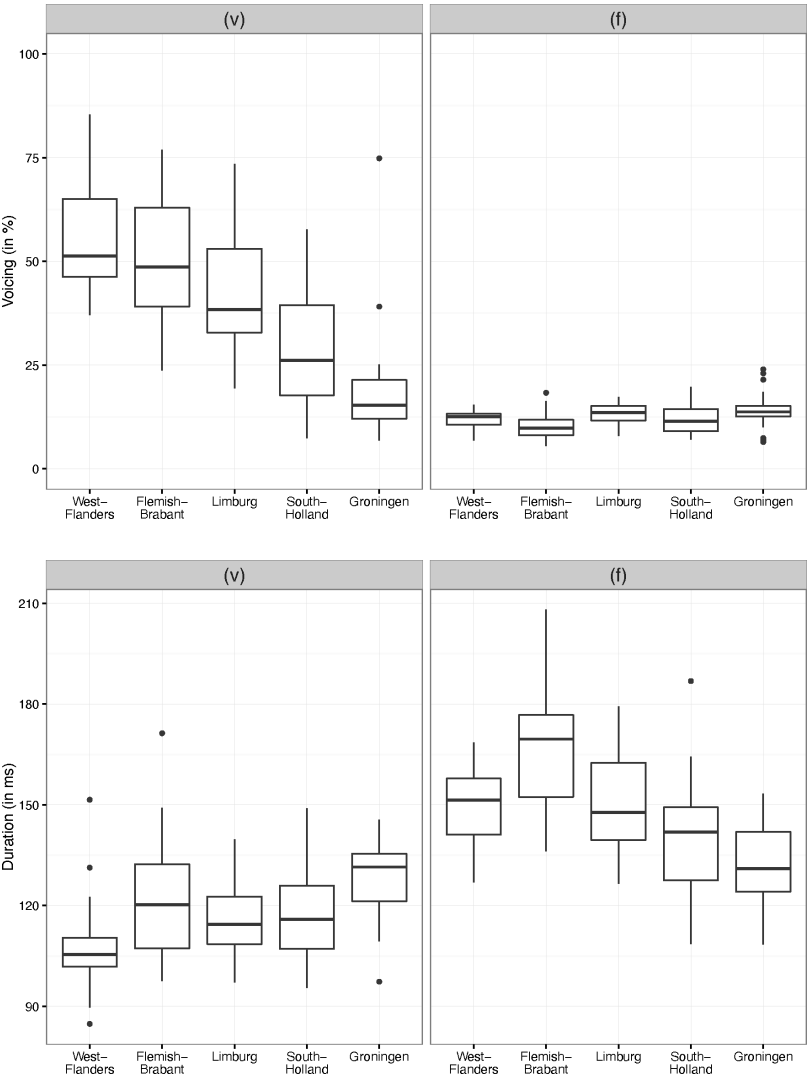
Figure 2: Boxplot of (v) and (f) with voicing (in %) (in the upper panel) and duration (in ms) (in the lower panel), divided by region.
