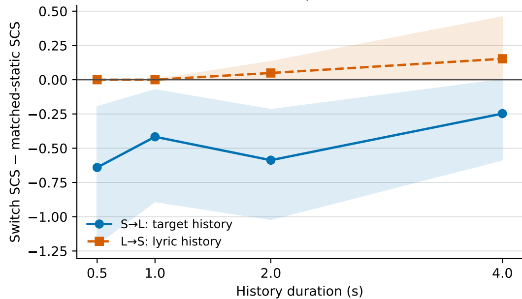
Whisper
