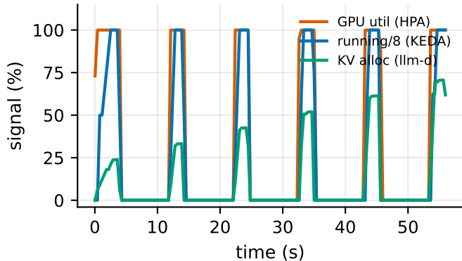
(a) All three signals read zero during tool calls
