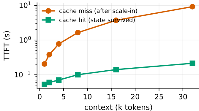
(b) Price of losing the state: 8.98 s at 32k context
