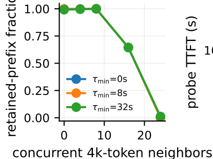
(c) pressure evicts state
