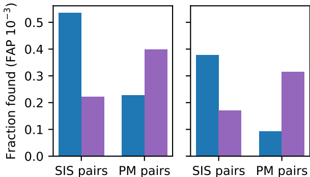
PI-ResNet
