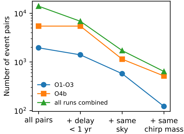
FIG. 5. Number of real event pairs after each physical requirement, for O1–O3, O4b and the combined catalogue (Table II).
