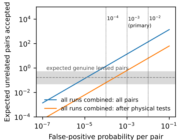
FIG. 7. Expected number of unrelated real pairs that a pair test would wrongly accept, as a function of its false-alarm probability per pair, for all 14 028 pairs of the combined O1–O3 and O4b catalogue (blue) and for the 637 pairs that pass the physical requirements (orange). The grey band shows the expected number of genuine lensed pairs, 0.05–0.5. Vertical lines mark the three operating points calibrated for PI-ResNet.
