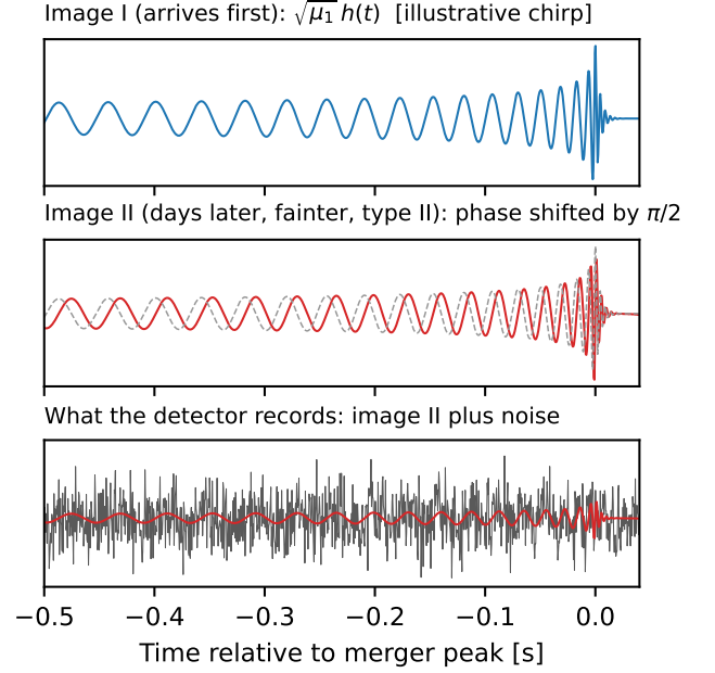
FIG. 1. What a pair test must recognise. Top: the first, brighter (type-I) image of an illustrative chirp. Middle: the second, fainter image of a type-II (saddle-point) image; the dashed grey curve shows the same signal without the \pi/2 Morse phase shift of Eq. (1). Bottom: the second image as it would appear in detector noise. PI-ResNet receives the two noisy segments, each normalised to unit variance, and must decide whether they are copies of one signal.
