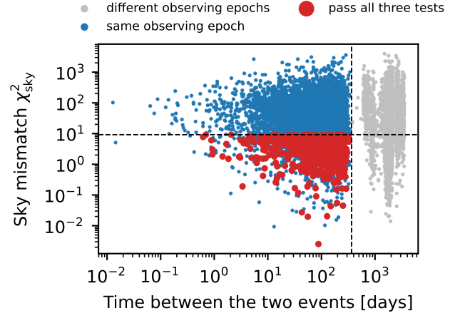
FIG. 6. All 14 028 real event pairs in the plane of time separation and sky mismatch. Grey: pairs from different observing epochs (O1–O3 versus O4b). Blue: pairs from the same epoch. Red: pairs that also pass the chirp-mass requirement. Dashed lines mark the one-year delay limit and the 99% sky-consistency limit.
