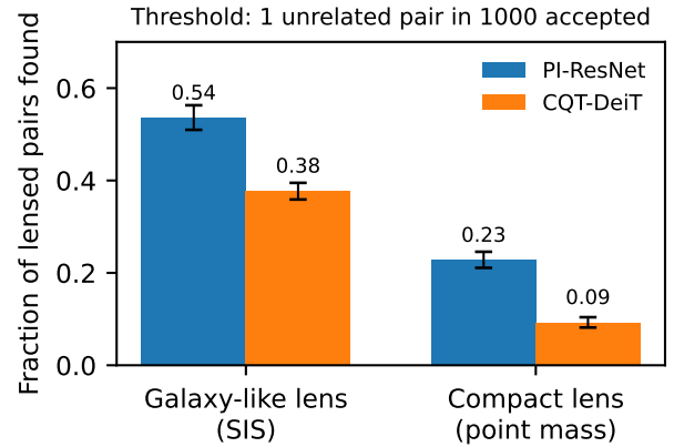
FIG. 2. Fraction of genuine lensed pairs recovered when the threshold is set so that one unrelated pair in a thousand is accepted ( p_{\text{FA}} = 10^{-3} ), measured on the independent catalogue B. Error bars are 95% ranges from resampling groups of sources.
