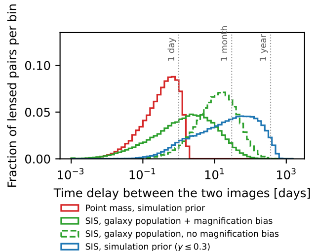
FIG. 4. Time delay between the two images of a strongly lensed binary black hole. Blue and red: the singular-isothermal-sphere and point-mass priors used to build the simulated catalogues. Green: singular isothermal spheres drawn from the observed galaxy population, without (dashed) and with (solid) the preference for well-aligned, highly magnified systems among detected pairs. Dotted lines mark one day, one month and one year.
