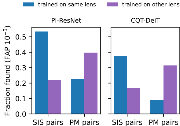
FIG. 3. Fraction of lensed pairs recovered at p_{\text{FA}} = 10^{-3} when the network is trained on the same lens model as the test pairs (blue) or on the other model (purple).
